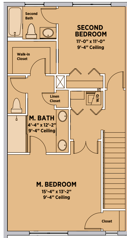
THIRD FLOOR PLAN 710 sf
